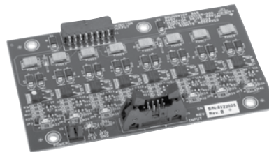
14100414000 Assembly - Injector Driver PCB
