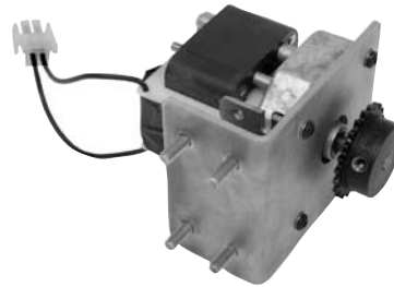
14100269115 Assembly - Dispersion Roller Motor, 115V 14100269230 Assembly - Dispersion Roller Motor, 230V With Electrical Connector
